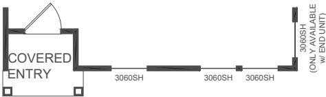
FIRST FLOOR
